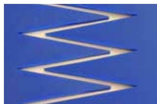
Finger joint with a hot press
