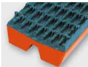
PU75A Twin V-belt (24 x 6,8 mm) with PVC Supergrip coating (CD-SG).
